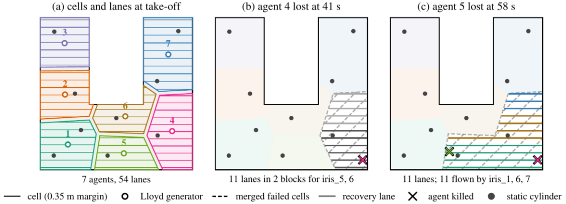
FIGURE 2. High-level planning in the PID-H_\infty U-shape mission, reproduced with the planner code (centroids within 0.6 cm of the log, identical lane counts). (a) Cells and their 54 lanes; first and last lanes follow the cell boundary. (b) Agent 4 is lost; its cell yields 11 lanes for agents 5, 6. (c) Helper 5 is lost too; the merged cells yield 11 lanes, coloured by the agent that flew them.
